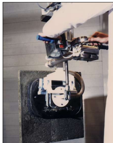
Vacuum Lifter - 90° rotation
